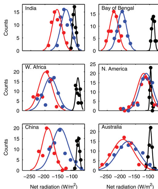
Fig. 6. State of current monsoon systems with respect to the critical point computed from the conceptual model. The black distribution reflects observed fluctuations in net radiation in the different monsoon systems. The blue distribution provides the computed critical threshold from the conceptual model. The red distribution includes the effect of evaporation. Lines give a Gaussian function with the same mean and standard deviation as the corresponding discrete distribution.
