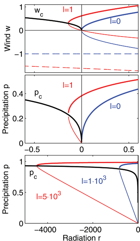
Fig. 5. Solution of the nondimensional governing Eq. 6. (Top) Nondimensional landward wind for two values of the only parameter l = 0 and l = 1 . (Middle) Corresponding nondimensional precipitation. (Bottom) Nondimensional precipitation for higher values of l as observed in some monsoon systems. The functional form of the solution is not changed qualitatively. The critical threshold ( w_c(l) , p_c(l) ) is given as the black curve in each frame.
